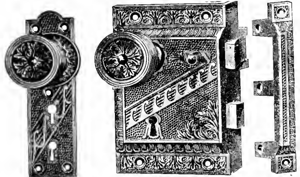
Figs. 2673-2674. COMBINED END-DOOR LOCK AND NIGHT-LATCH, KEEPER AND ESCUTCHEON-PLATE.
